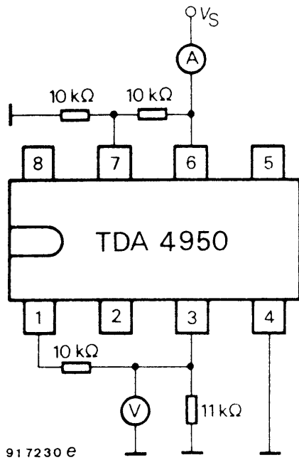
Figure 3 Test circuit 1
