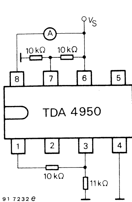
Figure 5 Test circuit 3
