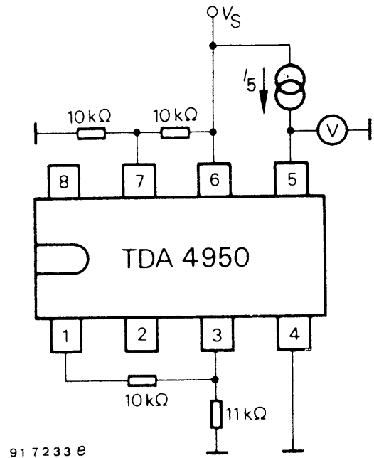
Figure 6 Test circuit 4
