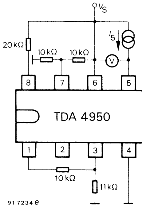
Figure 7 Test circuit 5
